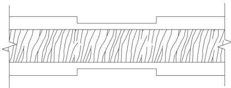
Groove Detail 9/16" wide x 1/16" deep
