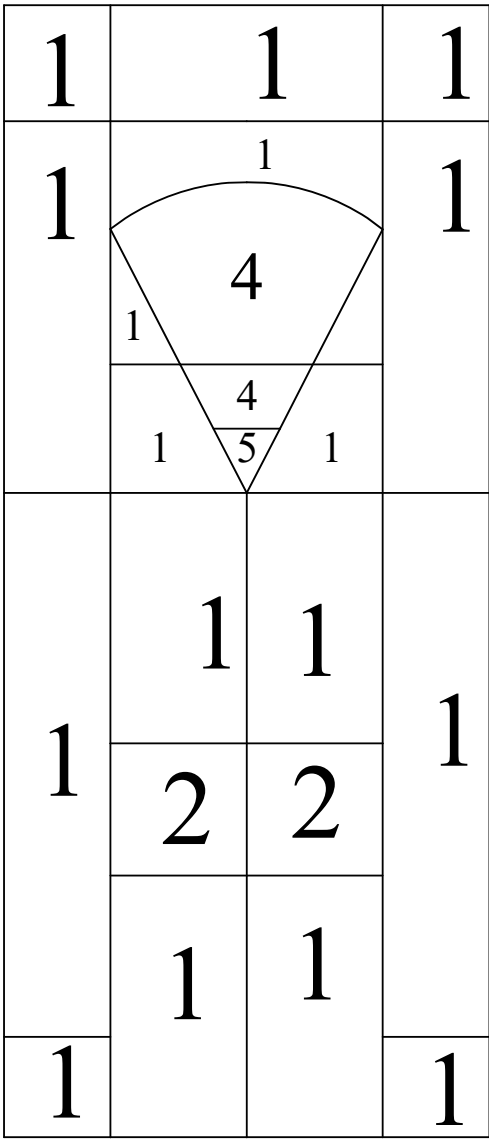
6181 SIDELITE GLASS SIZE: 7-7/8" x 18-3/8"
