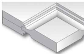
SCOOP PANEL WITH STEP-SHAKER STICKING
