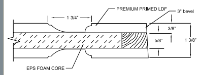
STANDARD 1-3/8" THICK DOOR
