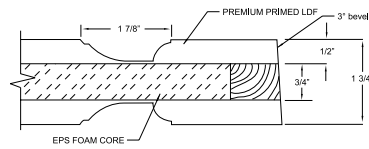
STANDARD 1-3/4" THICK DOOR
