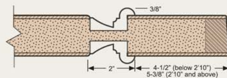
Flush Molding Profile
