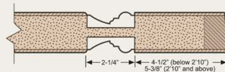
Flush Molding Profile
