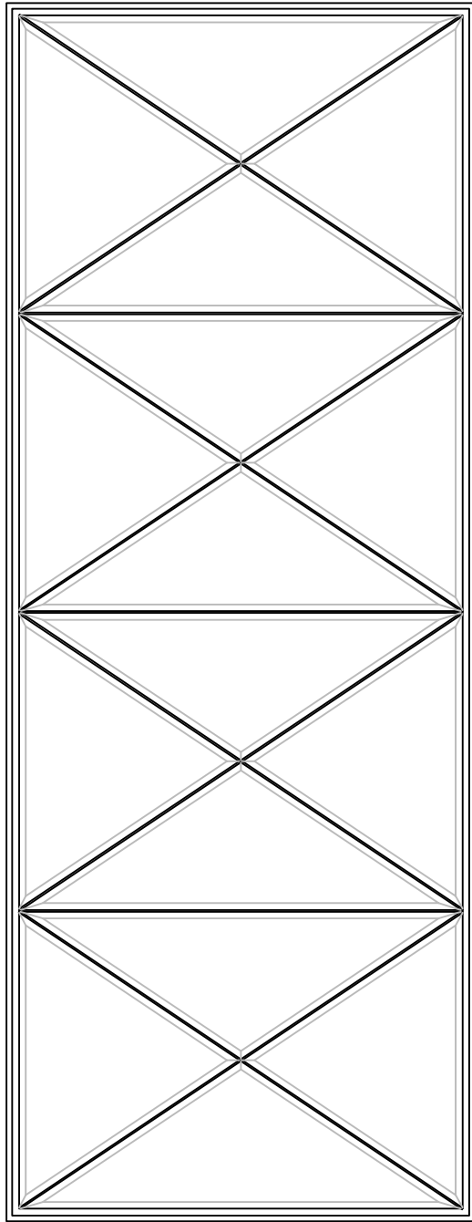
3-0 WATTSWORTH D/L IG : 25-7/8" x 67-1/4" x 3/4"
